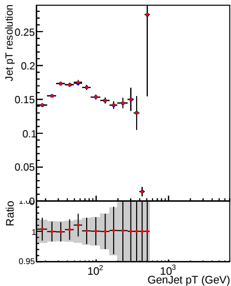
Raw Jet pT resolution using RMS, 3.0 < |\eta| < 5.0
