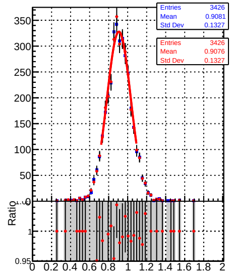
Raw Jet response (pT/pTgen) in 84 &lt;= pt &lt; 114, 1.3 &lt;= |eta| &lt; 2.1
