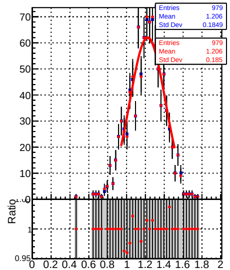
Raw Jet response (pT/pTgen) in 84 &lt;= pt &lt; 114, 3.0 &lt;= |eta| &lt; 5.0
