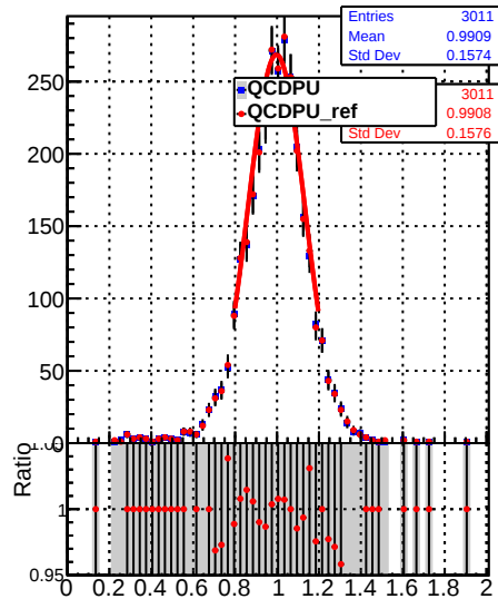
Jet response (pT/pTgen) in 64 \leq p_t < 84 , 0.5 \leq |\eta| < 0.5
