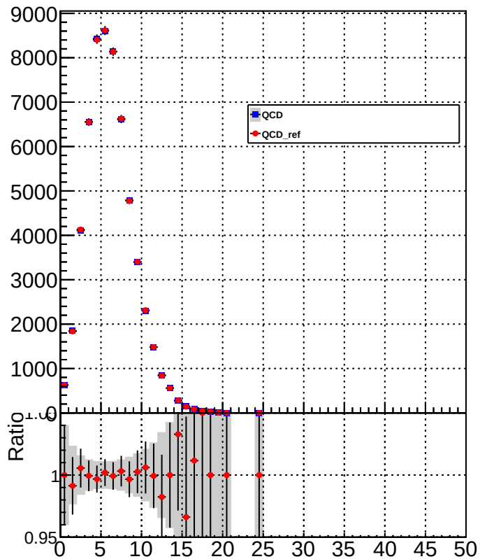
neutralHadronMultiplicity
