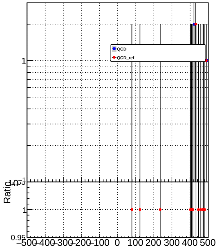
METResolution_GenMETTrue_MET400to500
