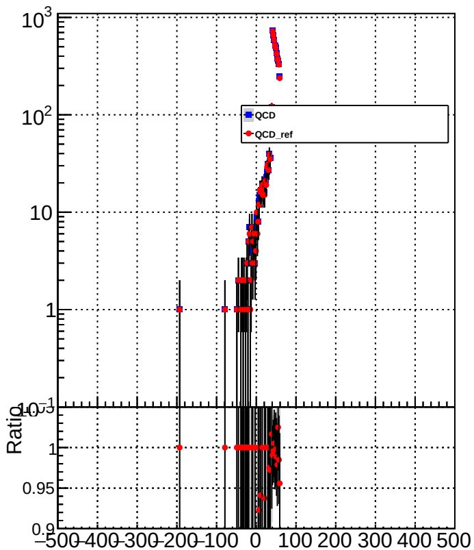
METResolution_GenMETTrue_MET40to60
