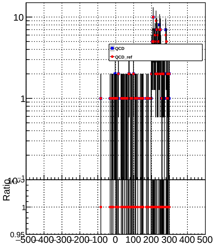
METResolution_GenMETTrue_MET200to300
