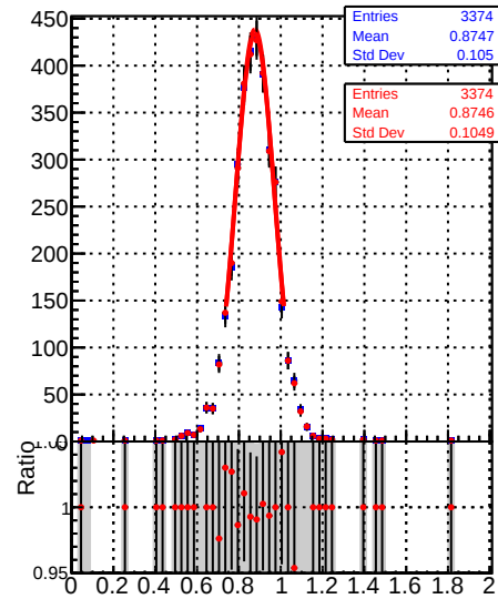
Raw Jet response ( p_T/p_{T\text{gen}} ) in 114 \leq p_t < 153 , 1.3 \leq |\eta| < 2.1
