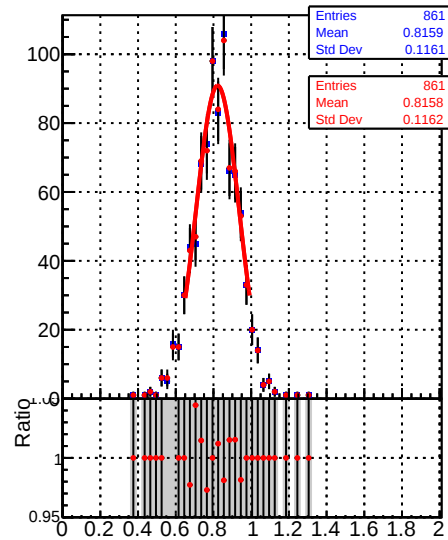
Raw Jet response ( p_T/p_{T\text{gen}} ) in 114 \leq p_t < 153 , 2.5 \leq |\eta| < 3.0
