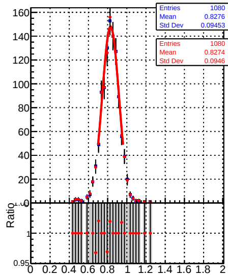
Raw Jet response ( p_T/p_{T\text{gen}} ) in 114 \leq p_t < 153 , 2.1 \leq |\eta| < 2.5
