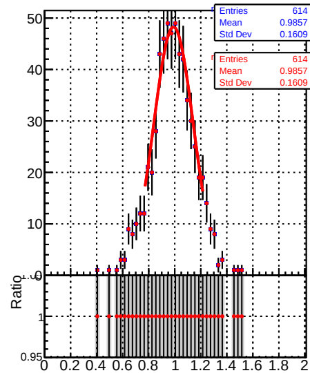
Raw Jet response ( p_T/p_{T\text{gen}} ) in 114 \leq p_t < 153 , 3.0 \leq |\eta| < 5.0
