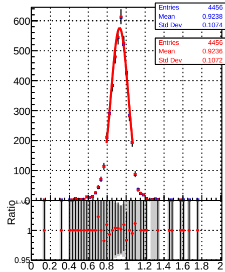
Raw Jet response ( p_T/p_{T\text{gen}} ) in 114 \leq p_t < 153 , 0.5 \leq |\eta| < 1.3
