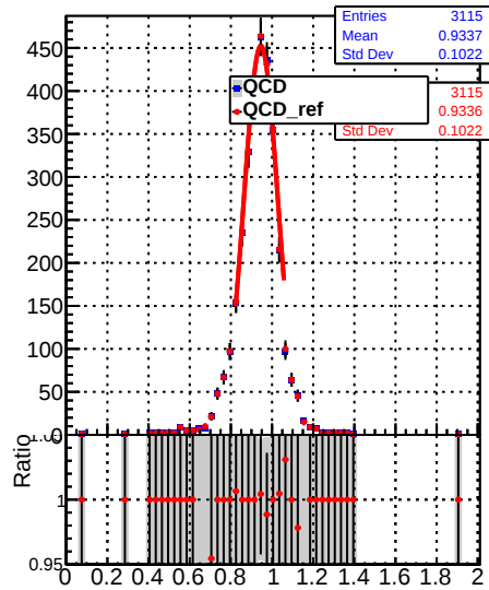
Raw Jet response ( p_T/p_{T\text{gen}} ) in 114 \leq p_t < 153 , 0.0 \leq |\eta| < 0.5
