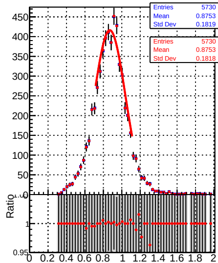
Raw Jet response (pT/pTgen) in 21 \leq p_t < 28, 0.5 \leq |\eta| < 1.3
