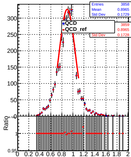
Raw Jet response (pT/pTgen) in 21 \leq p_t < 28, 0.0 \leq |\eta| < 0.5
