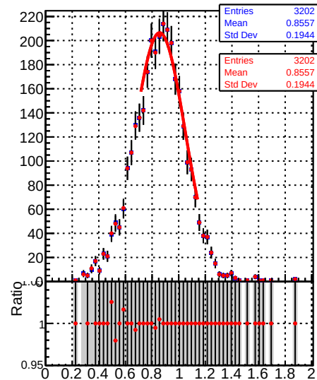
Raw Jet response (pT/pTgen) in 21 \leq p_t < 28, 3.0 \leq |\eta| < 5.0
