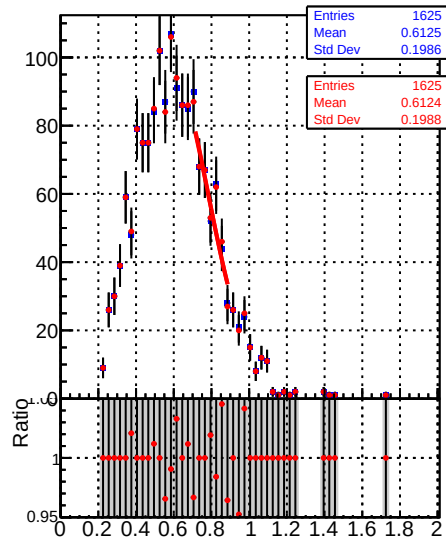
Raw Jet response (pT/pTgen) in 21 \leq p_t < 28, 2.5 \leq |\eta| < 3.0
