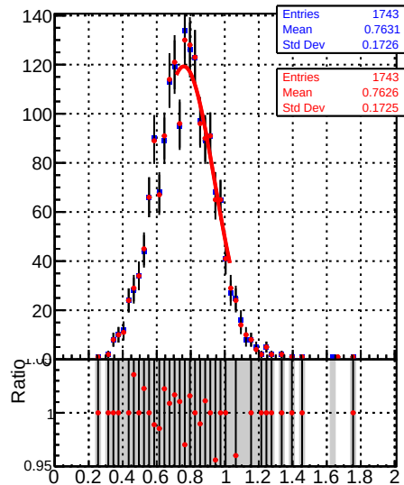
Raw Jet response (pT/pTgen) in 21 \leq p_t < 28, 2.1 \leq |\eta| < 2.5
