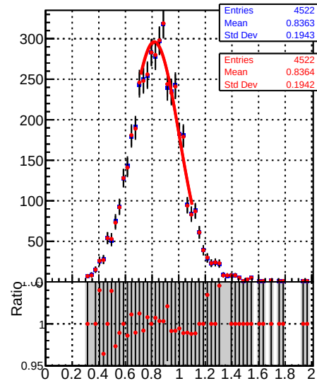
Raw Jet response (pT/pTgen) in 21 \leq p_t < 28, 1.3 \leq |\eta| < 2.1
