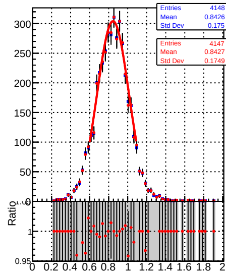
Raw Jet response (pT/pTgen) in 28 \leq p_t < 37 , 1.3 \leq |\eta| < 2.1
