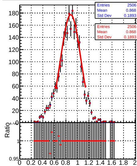
Raw Jet response (pT/pTgen) in 28 \leq p_t < 37 , 3.0 \leq |\eta| < 5.0
