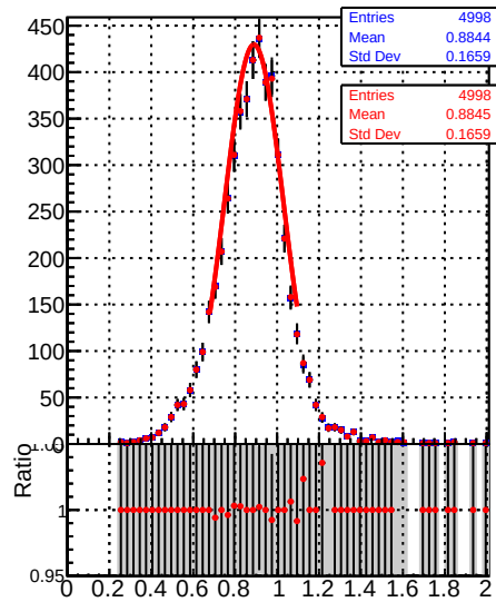
Raw Jet response (pT/pTgen) in 28 \leq p_t < 37 , 0.5 \leq |\eta| < 1.3
