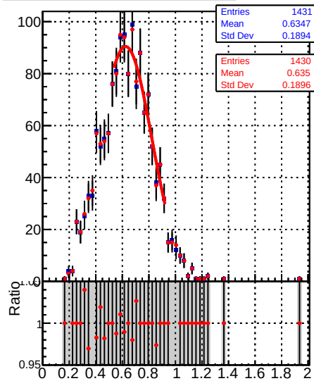
Raw Jet response (pT/pTgen) in 28 \leq p_t < 37 , 2.5 \leq |\eta| < 3.0
