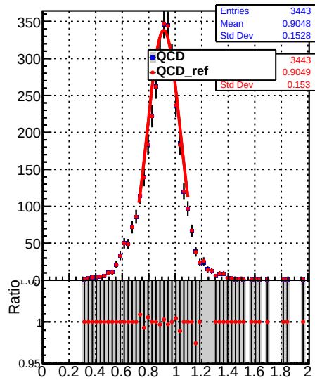
Raw Jet response (pT/pTgen) in 28 \leq p_t < 37 , 0.0 \leq |\eta| < 0.5
