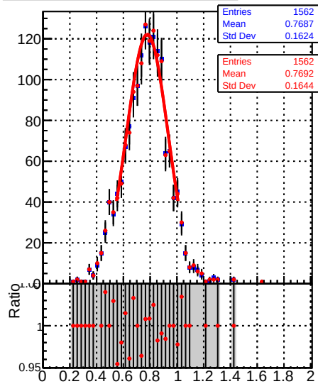
Raw Jet response (pT/pTgen) in 28 \leq p_t < 37 , 2.1 \leq |\eta| < 2.5
