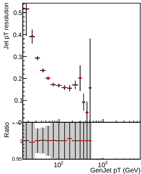
Raw Jet pT resolution, 3.0 < |\eta| < 5.0
