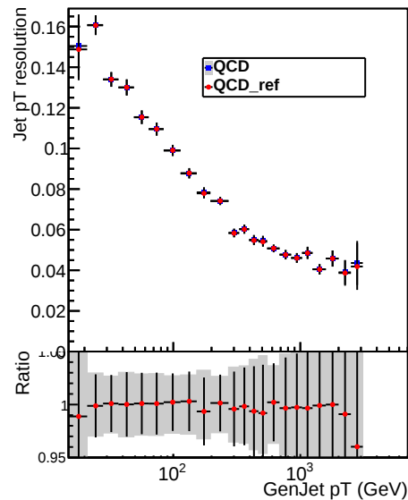
Raw Jet pT resolution, 2.1 < |\eta| < 2.5
