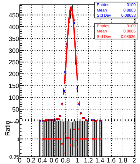
Raw Jet response (pT/pTgen) in 196 \leq p_t < 272 , 1.3 \leq |\eta| < 2.1
