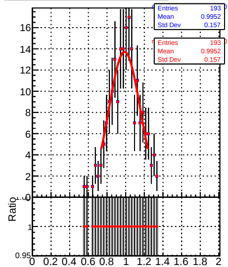
Raw Jet response (pT/pTgen) in 196 \leq p_t < 272 , 3.0 \leq |\eta| < 5.0
