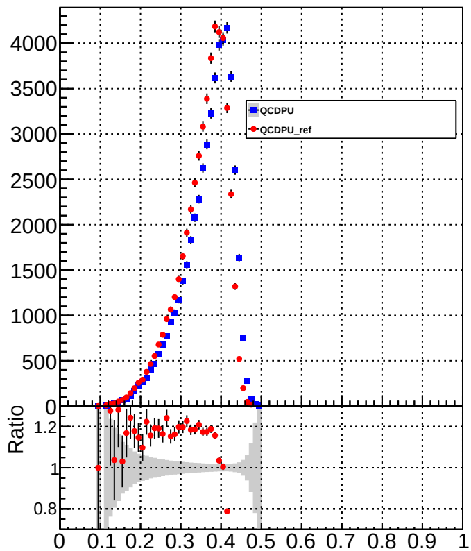
HFHadronEtFraction
