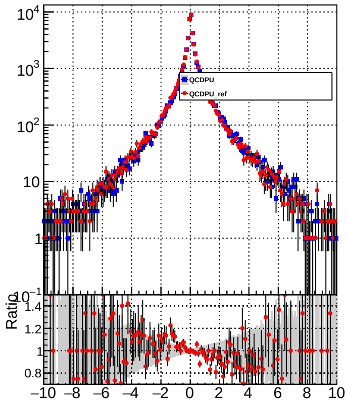
METUnc_PhotonEnDown
