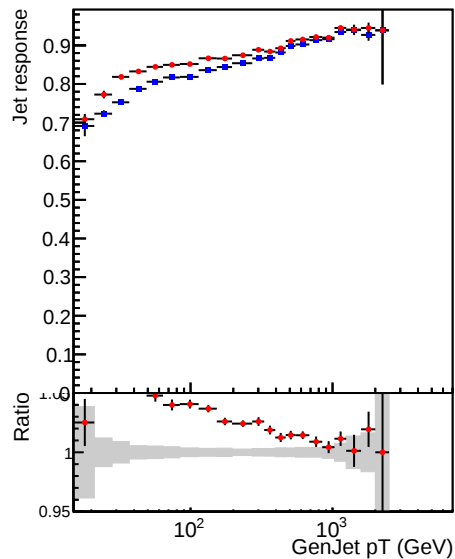
Raw Jet pT response, 3.0 < |\eta| < 5.0
