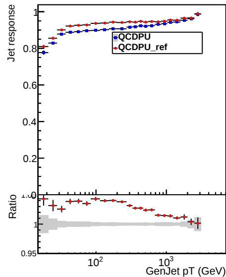
Raw Jet pT response, 2.1 < |\eta| < 2.5
