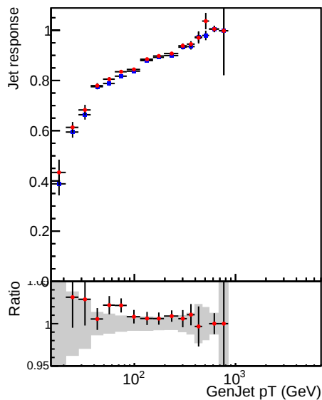
Raw Jet pT response, 2.5 < |\eta| < 3.0
