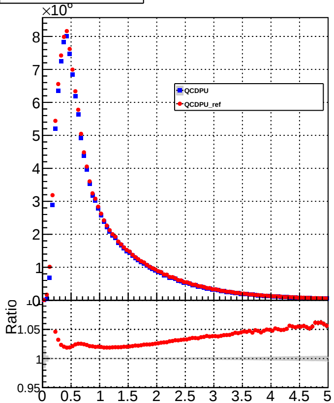
AllCandidatePtLow
