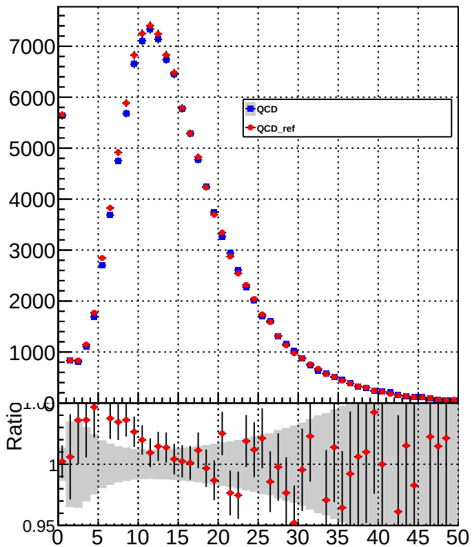
chargedHadronMultiplicity
