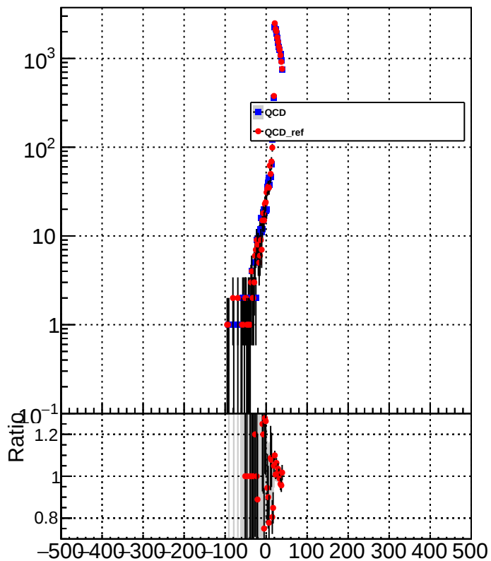
METResolution_GenMETTrue_MET20to40
