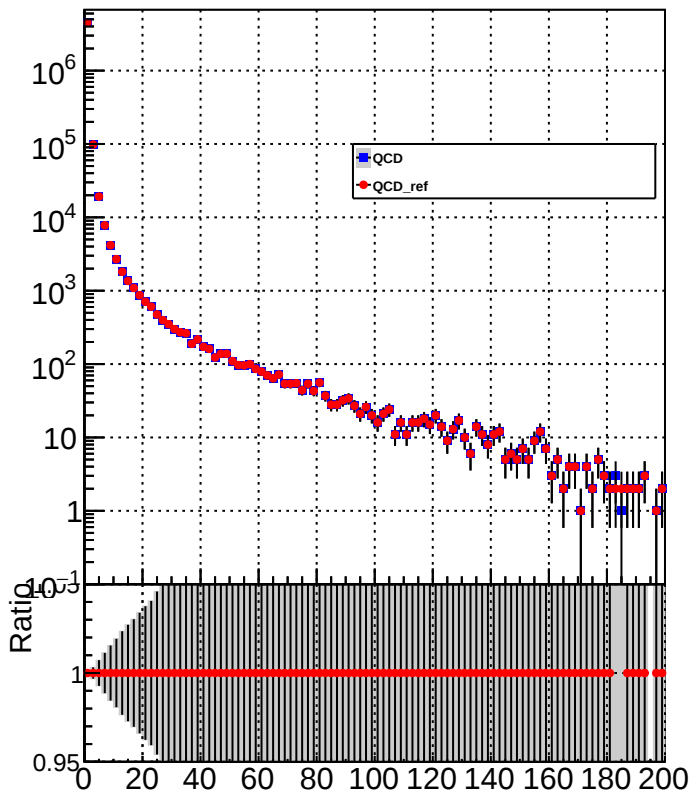
HF_hadronPtMid
