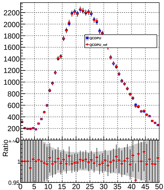
chargedHadronMultiplicity
