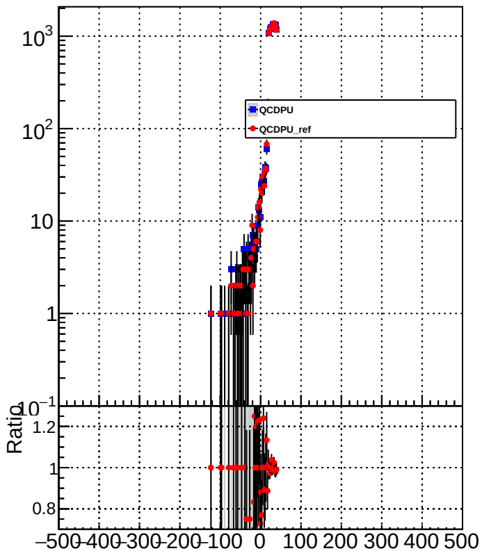
METResolution_GenMETTrue_MET20to40
