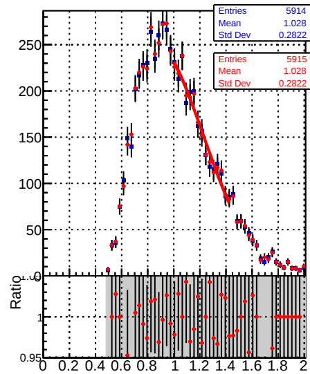
Jet response ( p_T/p_{Tgen} ) in 15 \leq p_T < 21 , 0.5 \leq |\eta| < 2.1
