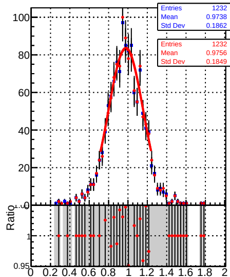
Jet response (pT/pTgen) in 64 \leq p_t < 84, 2.1 \leq |\eta| < 2.5
