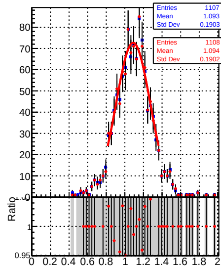
Jet response (pT/pTgen) in 64 \leq p_t < 84, 3.0 \leq |\eta| < 5.0
