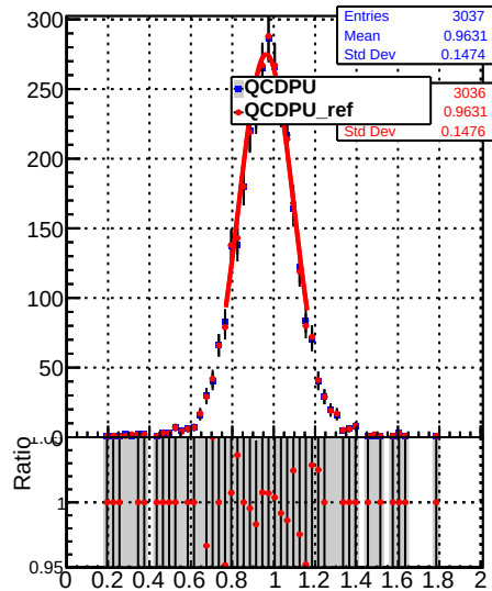
Jet response (pT/pTgen) in 64 \leq p_t < 84, 0.0 \leq |\eta| < 0.5
