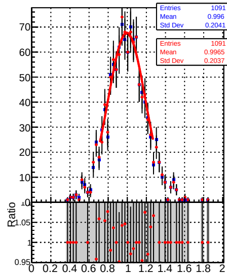
Jet response (pT/pTgen) in 64 \leq p_t < 84, 2.5 \leq |\eta| < 3.0
