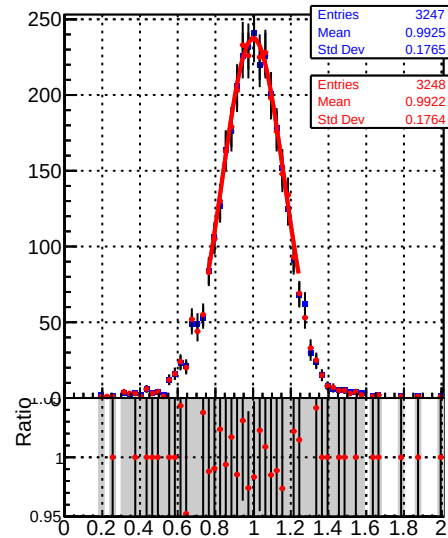
Jet response (pT/pTgen) in 64 \leq p_t < 84, 1.3 \leq |\eta| < 2.1
