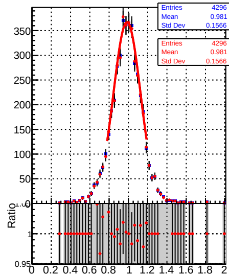
Jet response (pT/pTgen) in 64 \leq p_t < 84, 0.5 \leq |\eta| < 1.3
