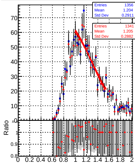
Raw Jet response (pT/pTgen) in 15 \leq p_t < 21, 2.1 \leq |\eta| < 2.5
