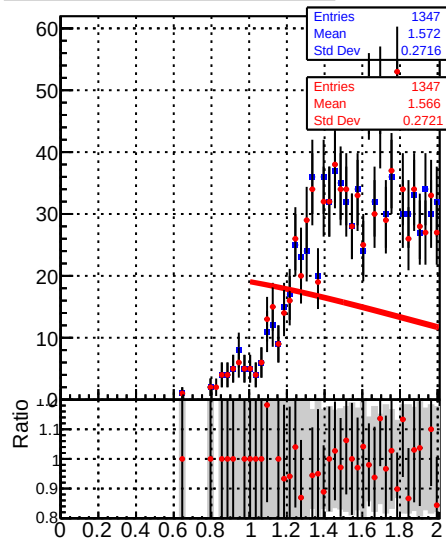
Raw Jet response (pT/pTgen) in 15 \leq p_t < 21, 2.5 \leq |\eta| < 3.0
