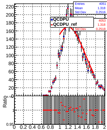
Raw Jet response (pT/pTgen) in 15 \leq p_t < 21, 0.0 \leq |\eta| < 0.5
