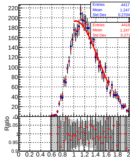
Raw Jet response (pT/pTgen) in 15 \leq p_t < 21, 1.3 \leq |\eta| < 2.1
