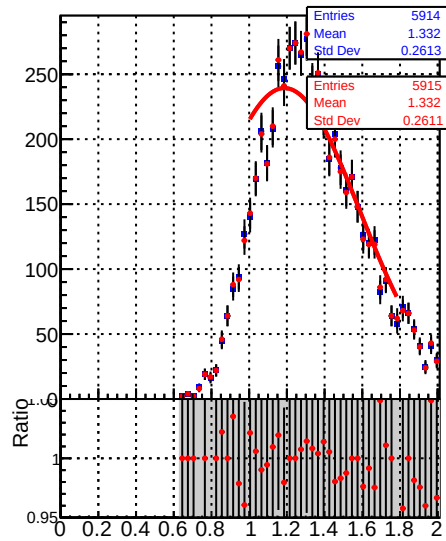
Raw Jet response (pT/pTgen) in 15 \leq p_t < 21, 0.5 \leq |\eta| < 2.1
