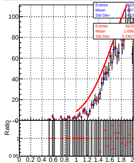
Raw Jet response (pT/pTgen) in 15 \leq p_t < 21, 3.0 \leq |\eta| < 5.0
