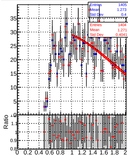
Jet response (pT/pTgen) in 15 \leq p_T < 21, 2.5 \leq |\eta| < 3.0
