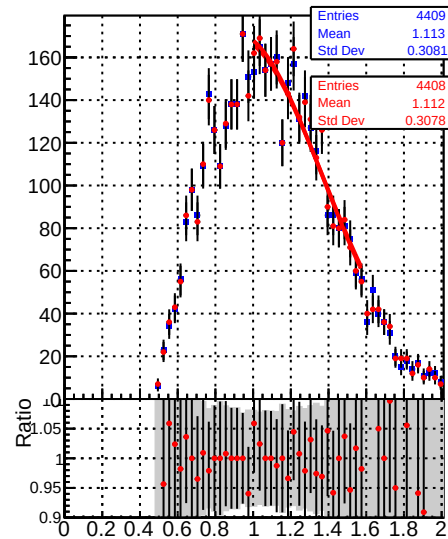
Jet response (pT/pTgen) in 15 \leq p_T < 21, 1.3 \leq |\eta| < 2.1
