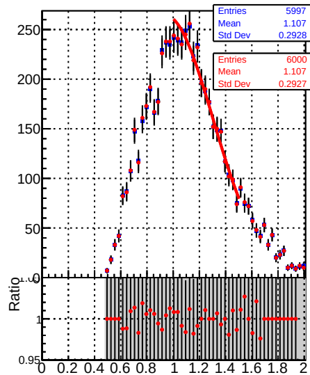
Jet response (pT/pTgen) in 15 \leq p_T < 21, 0.5 \leq |\eta| < 1.3
