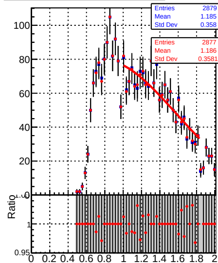
Jet response (pT/pTgen) in 15 \leq p_T < 21, 3.0 \leq |\eta| < 5.0
