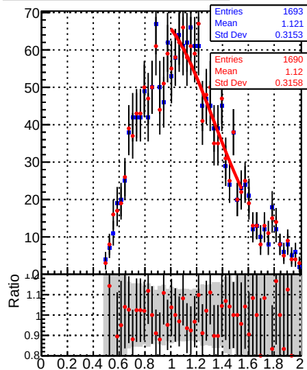
Jet response (pT/pTgen) in 15 \leq p_T < 21, 2.1 \leq |\eta| < 2.5
