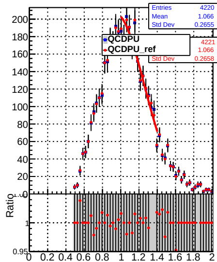
Jet response (pT/pTgen) in 15 \leq p_T < 21, 0.0 \leq |\eta| < 0.5
