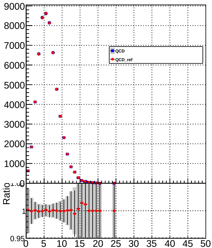
neutralHadronMultiplicity
