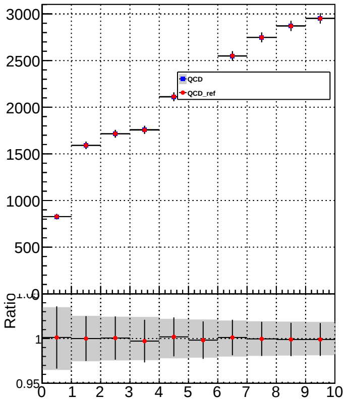
photonMultiplicity
