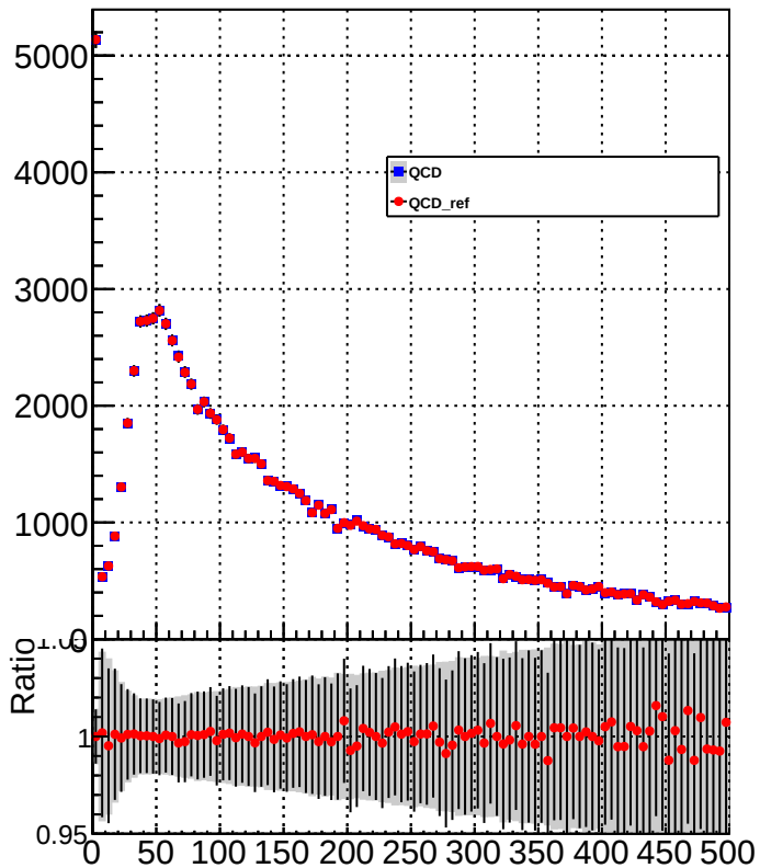
chargedHadronEnergy
