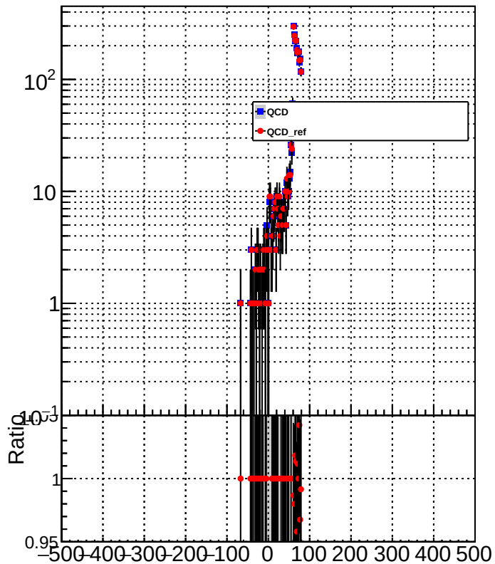
METResolution_GenMETTrue_MET60to80
