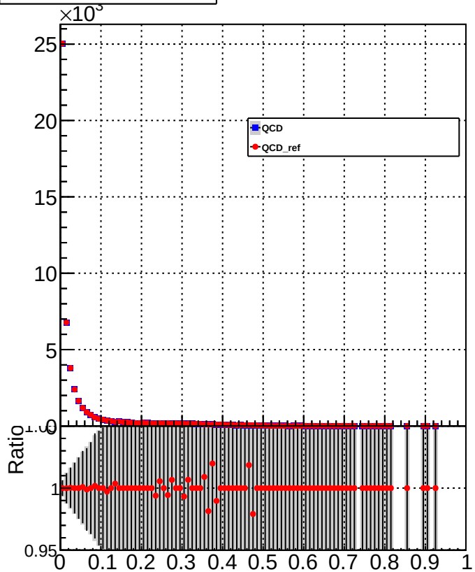
HFHadronEtFraction
