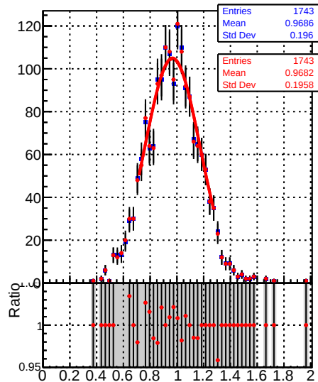
Jet response ( p_T/p_{T\text{gen}} ) in 21 \leq p_t < 28, 2.1 \leq |\eta| < 2.5
