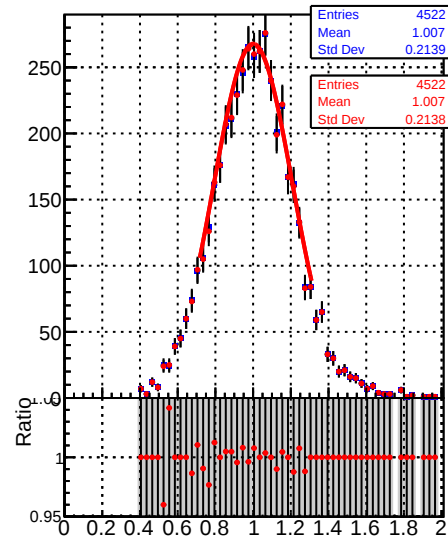
Jet response ( p_T/p_{T\text{gen}} ) in 21 \leq p_t < 28, 1.3 \leq |\eta| < 2.1
