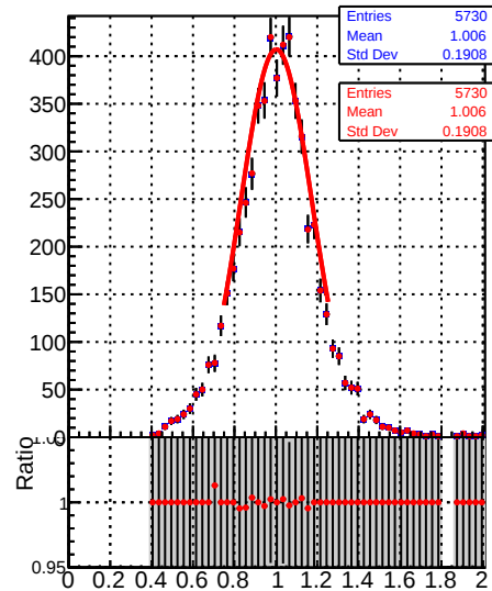
Jet response ( p_T/p_{T\text{gen}} ) in 21 \leq p_t < 28, 0.5 \leq |\eta| < 1.3
