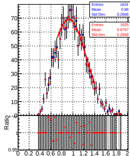
Jet response ( p_T/p_{T\text{gen}} ) in 21 \leq p_t < 28, 2.5 \leq |\eta| < 3.0
