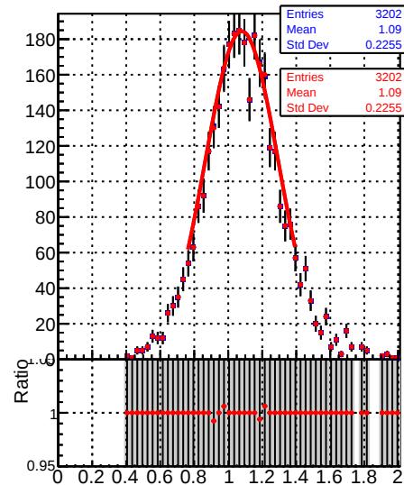
Jet response ( p_T/p_{T\text{gen}} ) in 21 \leq p_t < 28, 3.0 \leq |\eta| < 5.0
