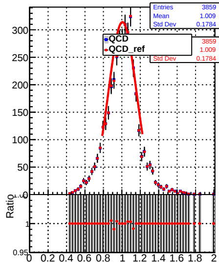
Jet response ( p_T/p_{T\text{gen}} ) in 21 \leq p_t < 28, 0.0 \leq |\eta| < 0.5
