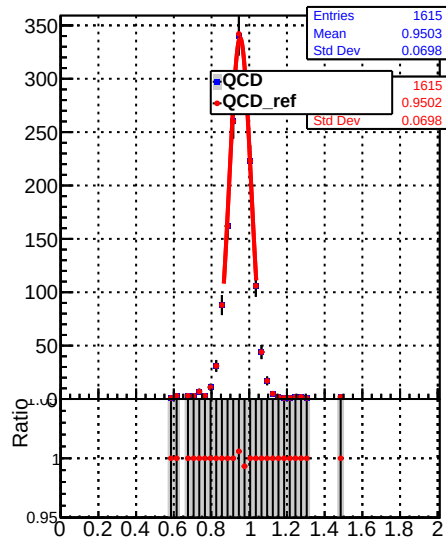
Raw Jet response (pT/pTgen) in 330 &lt;= pt &lt; 395, 0.0 &lt;= |eta| &lt; 2.5
