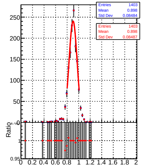
Raw Jet response (pT/pTgen) in 330 &lt;= pt &lt; 395, 1.3 &lt;= |eta| &lt; 2.1
