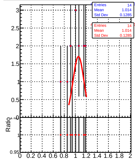
Raw Jet response (pT/pTgen) in 330 &lt;= pt &lt; 395, 3.0 &lt;= |eta| &lt; 5.0
