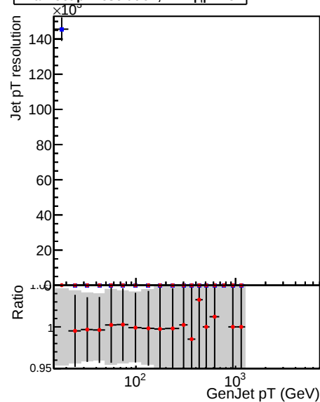
Raw Jet pT resolution, 2.1 < |\eta| < 2.5
