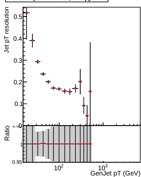
Raw Jet pT resolution, 3.0 < |\eta| < 5.0
